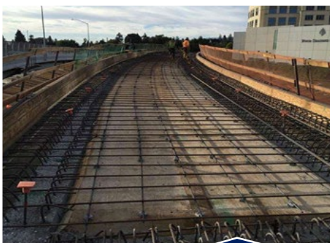
Placement of Deck Rebar
