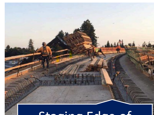
Staging Edge of Deck Forms
