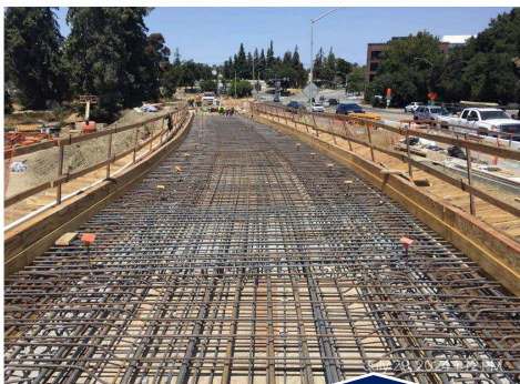
Bride Deck Construction
